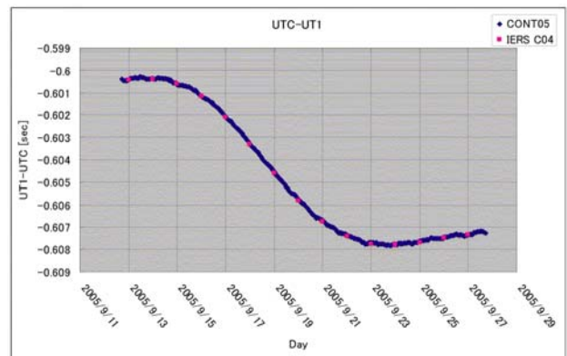
図-6 UT1-UTC ( cont05 )
