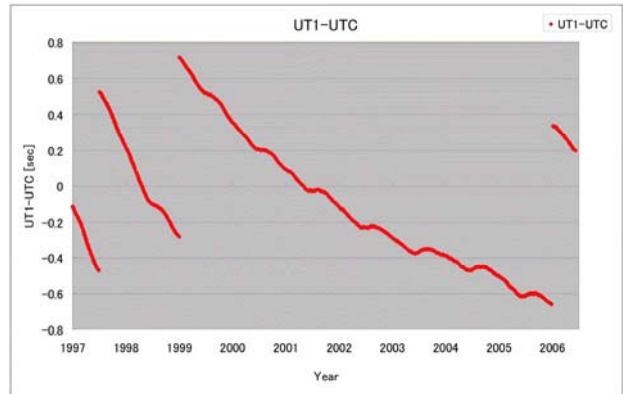
図-4 UT1-UTC ( int2006b )
