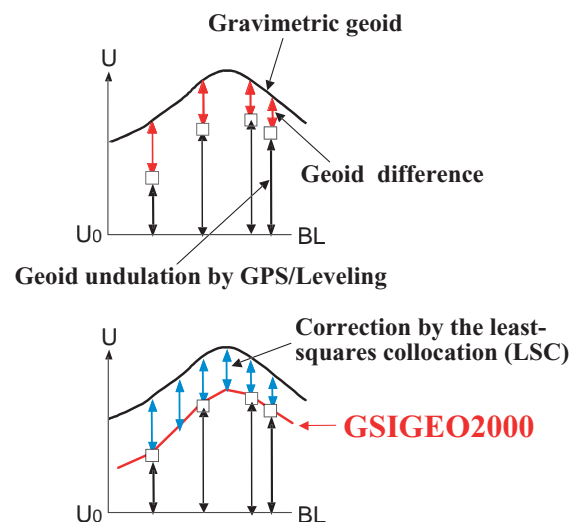
Fig. 4 Schematic diagram of hybrid geoid model construction.
