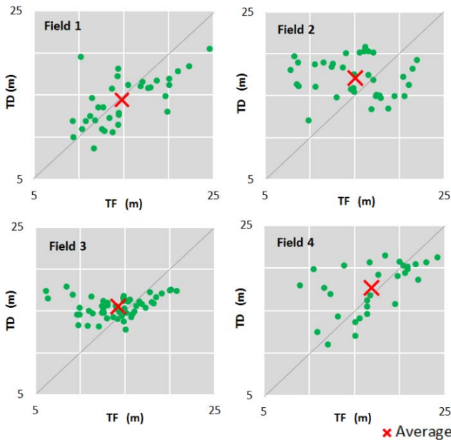
Fig. 4 Individual tree height for broadleaf deciduous forests in the Izumozaki region (green dots). TF: Tree height of field data, TD: Tree height estimated from corrected 1-m DCM.
