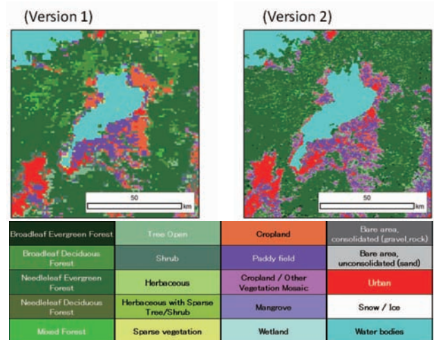
Fig.4 Global Map Global Version (Land Cover) around the Lake Biwa in Japan
