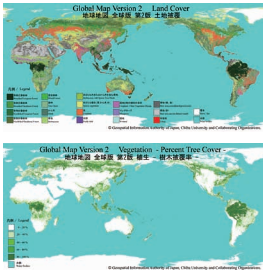
Fig.3 Global Map Global Version (Version 2): Land Cover and Vegetation
