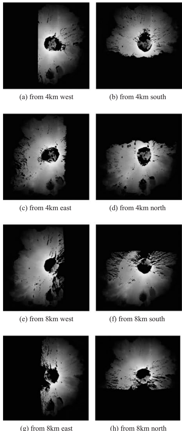
Fig. 7 Incomplete DEMs for 8 observations.
